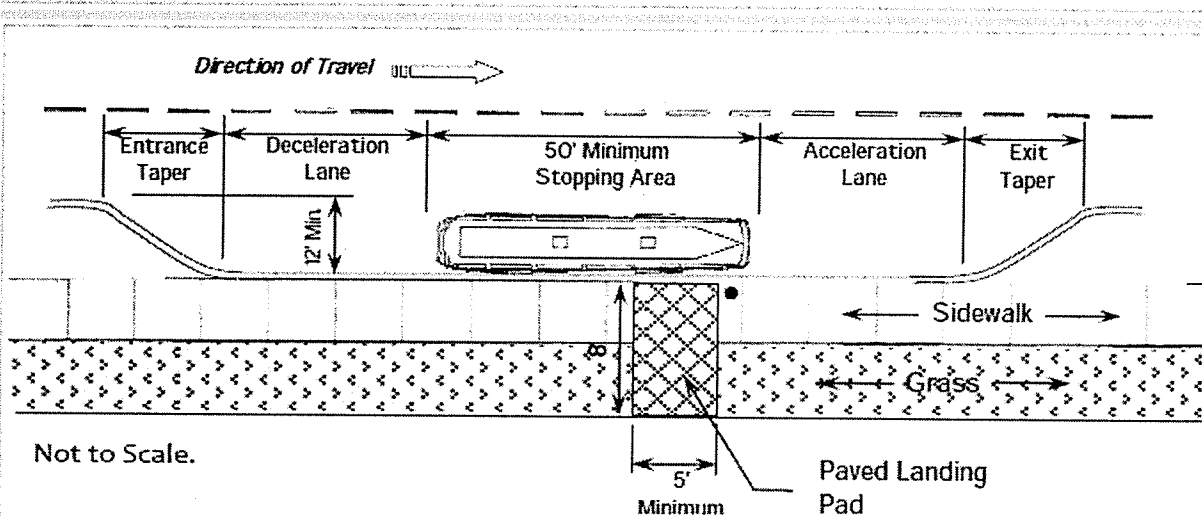
Figure 8. Parallel Bus Bay
